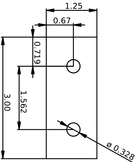
JAW MOUNTING AREA
